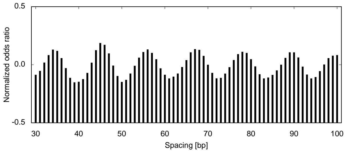
Spacings histogram after subtracting a fitted parabola
