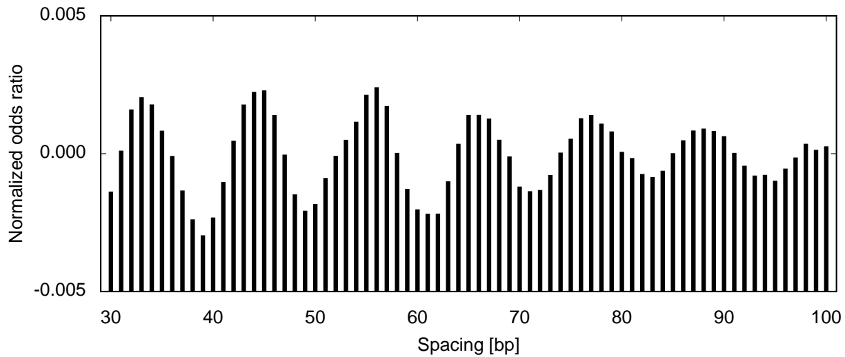
Spacings histogram after subtracting a fitted parabola
